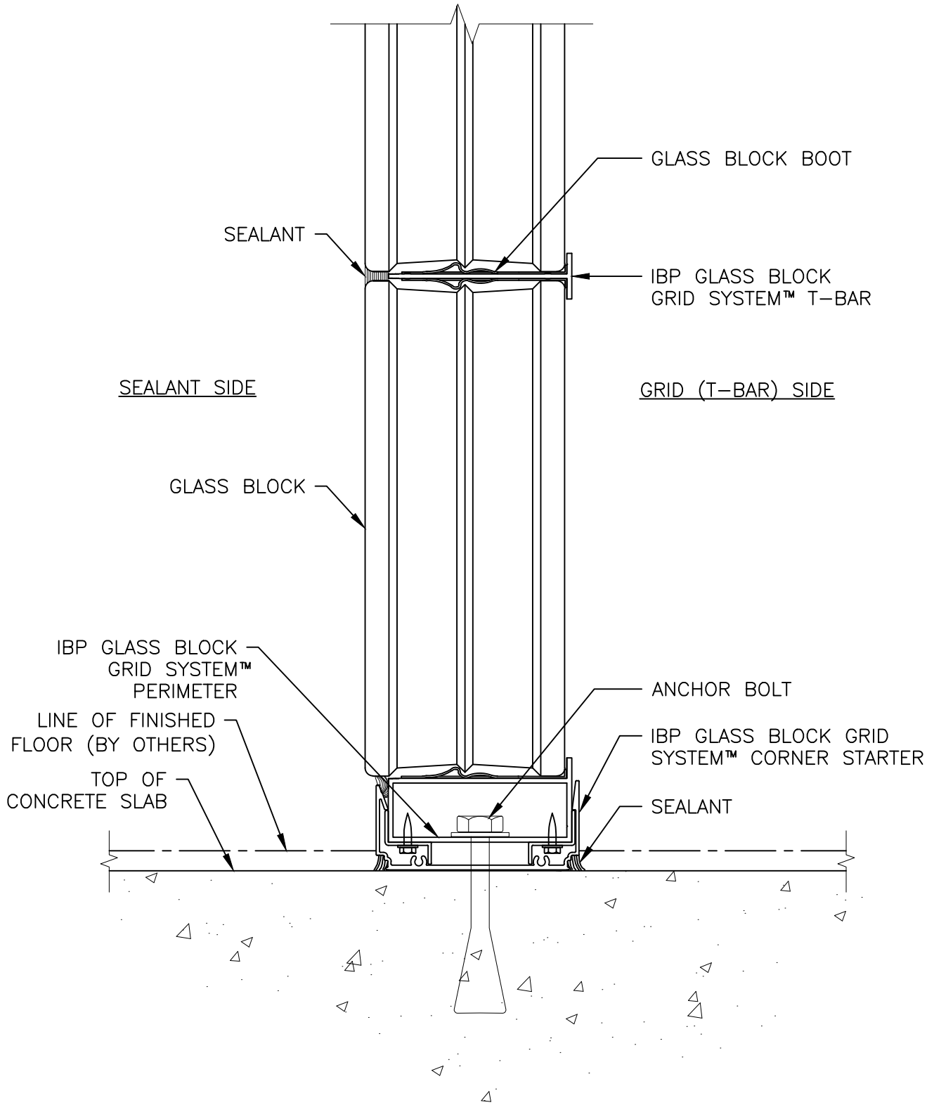
INTERIOR PARTITION AT FLOOR NOT TO SCALE
