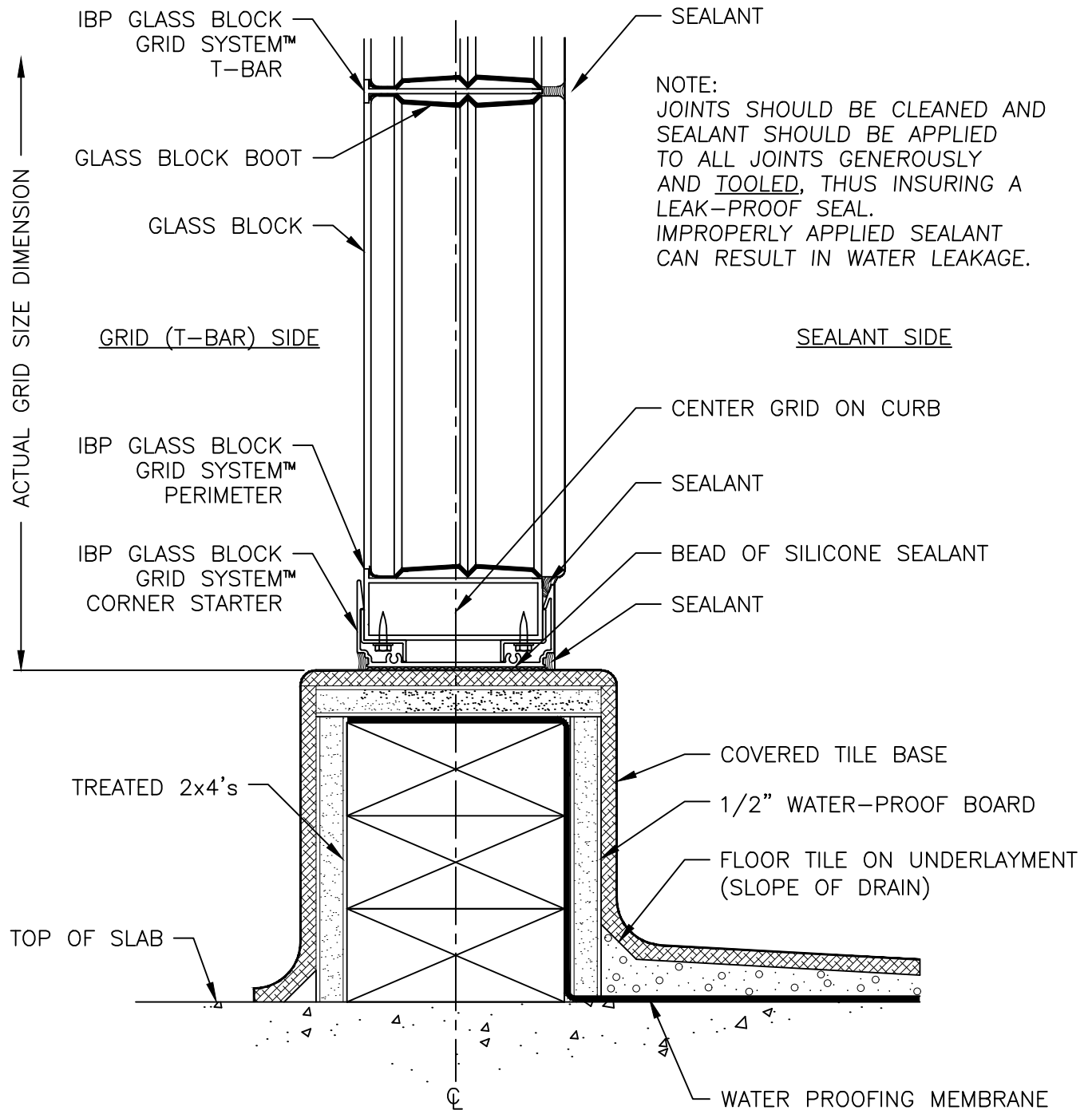
SHOWER CURB DETAIL THREE PLATE CURB – WOOD CONSTRUCTION NOT TO SCALE
