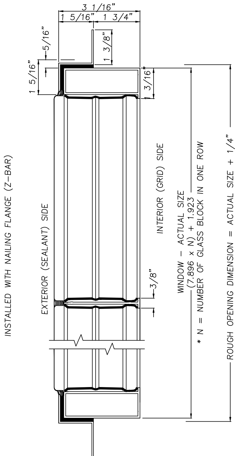
IBP GRID SYSTEM DIMENSIONS - WITH Z-BAR NOT TO SCALE
