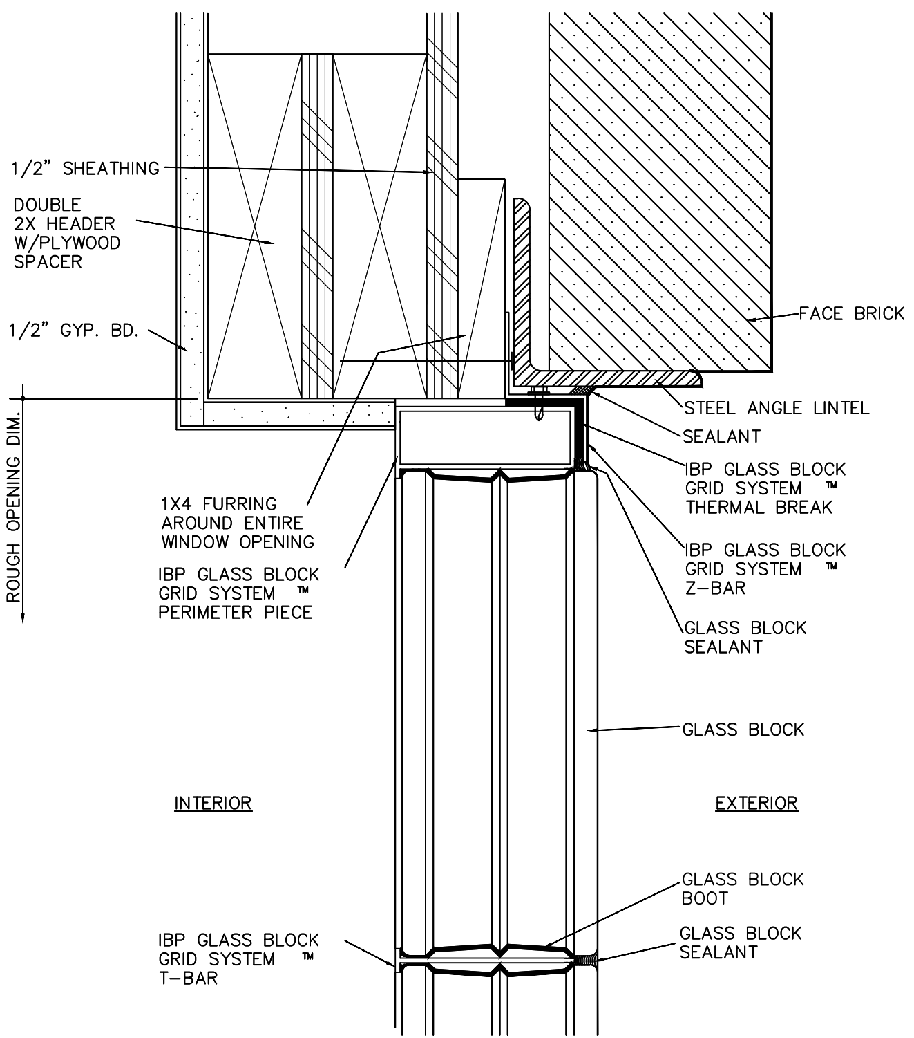
WINDOW HEAD – WOOD STUD/BRICK VENEER NOT TO SCALE
