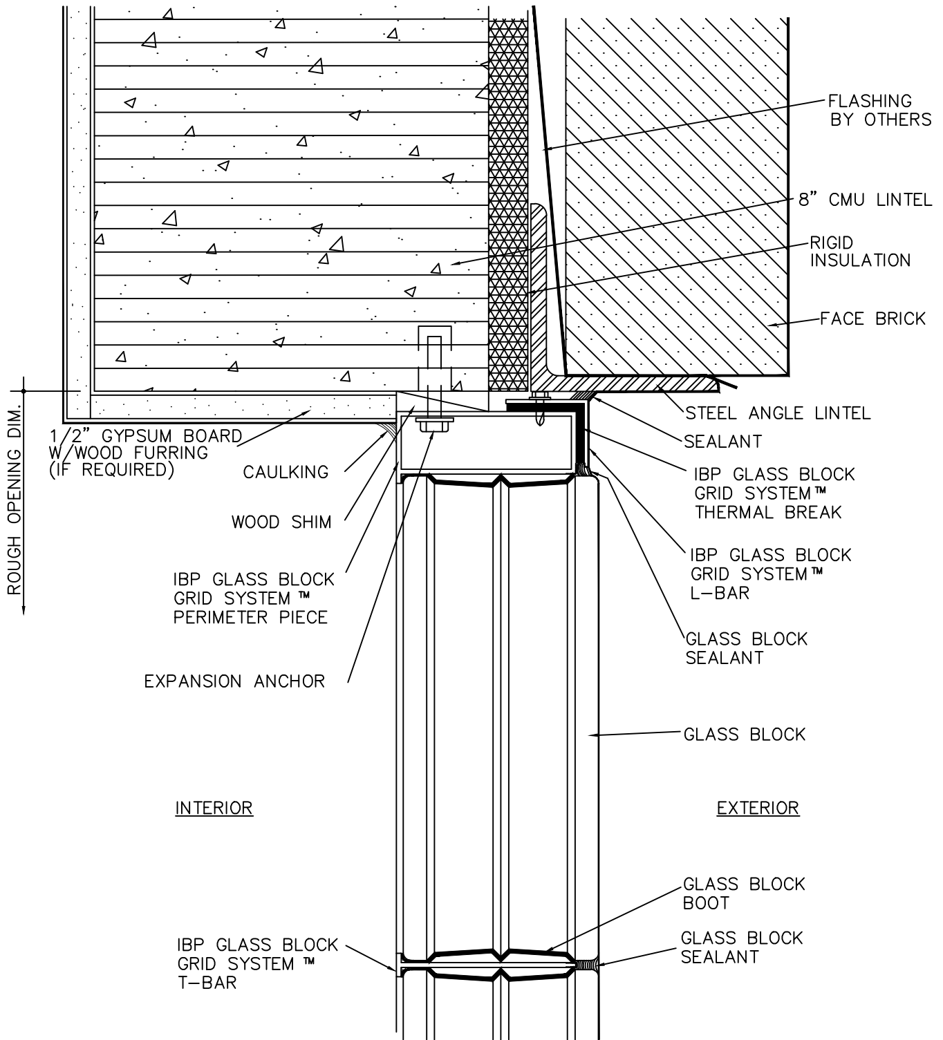
WINDOW HEAD – CMU WALL/BRICK VENEER NOT TO SCALE
