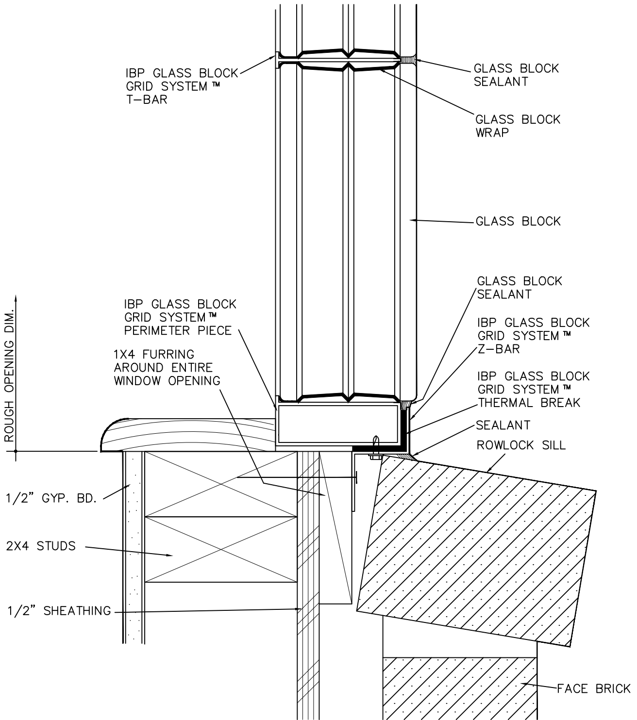
WINDOW SILL – WOOD STUD/BRICK VENEER NOT TO SCALE
