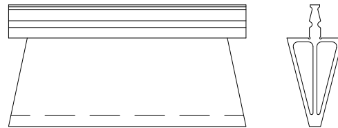
SPANNING/SPACER MEMBER SECTION AND PROFILE
