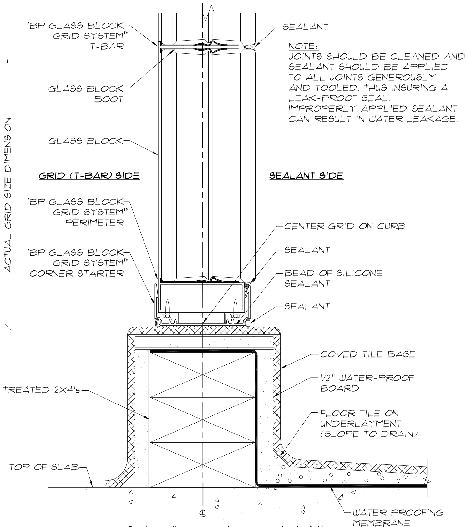
SHOWER CURB DETAIL THREE PLATE CURB - WOOD CONSTRUCTION SCALE: N.T.S.
