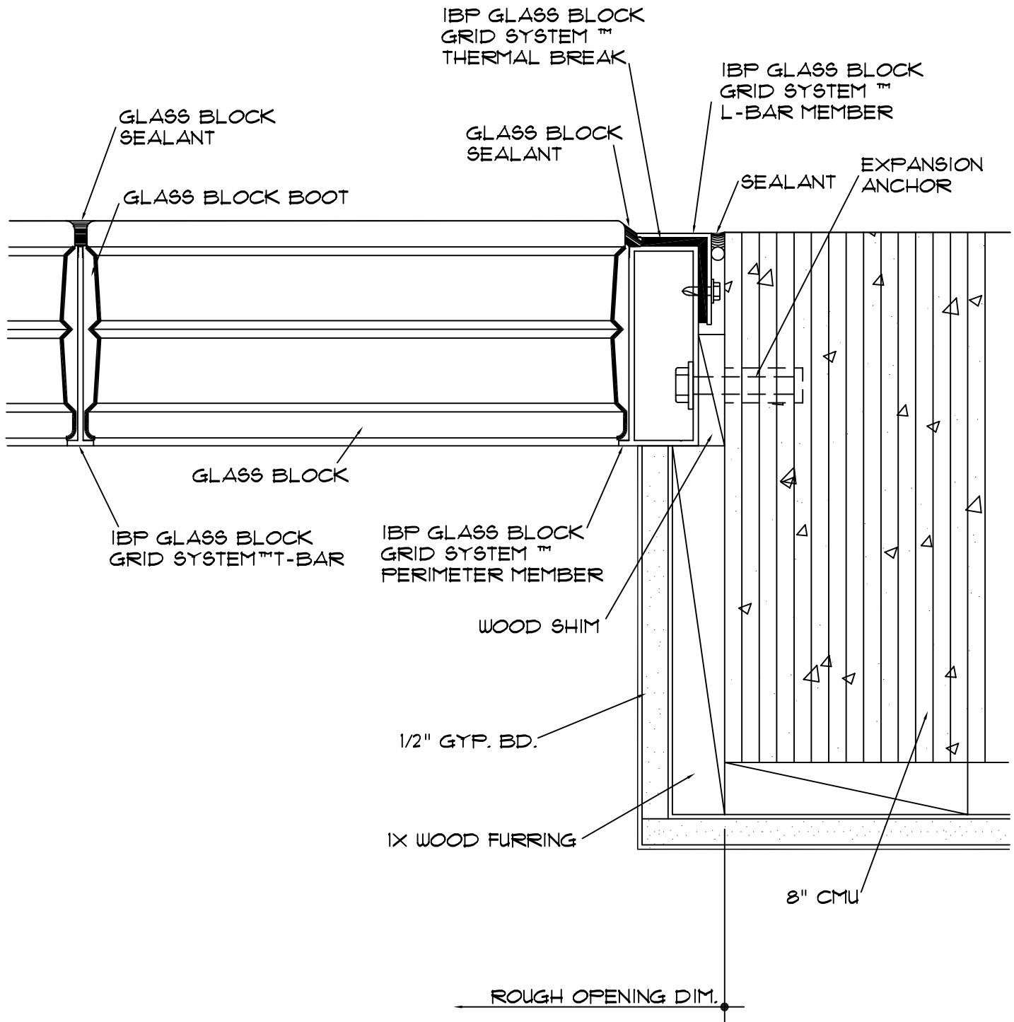
WINDOW JAMB - CMU WALL 1/2 FULL SCALE
